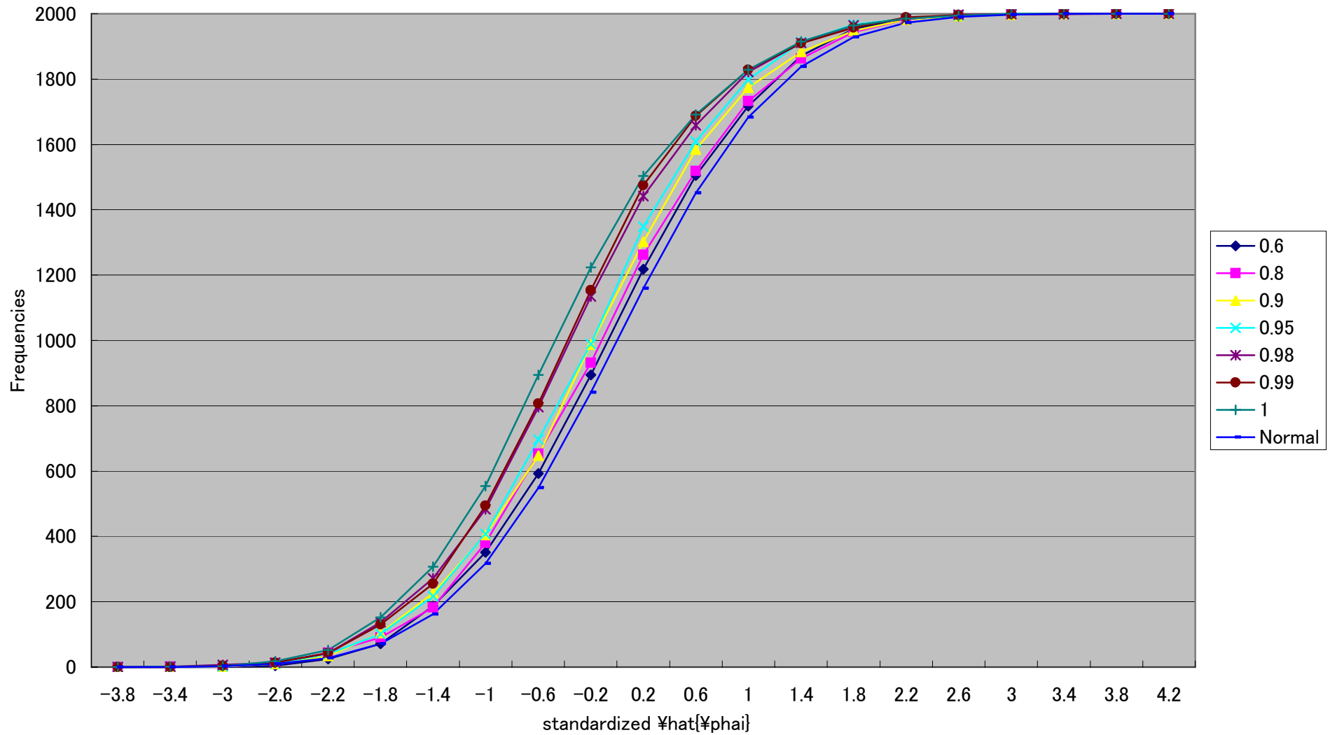
Empirical Distribution Function of standardized \hat{\varphi}
