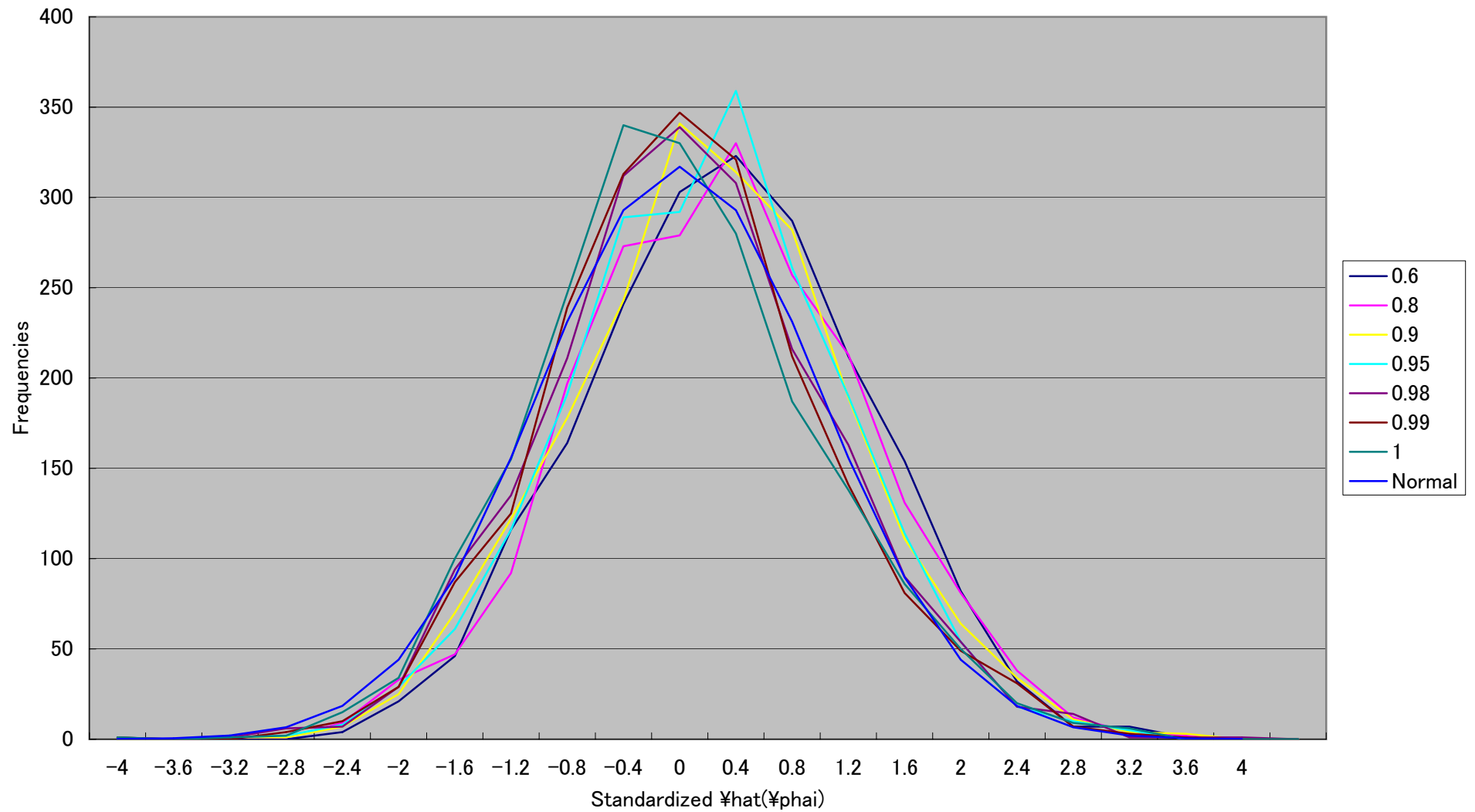
Empirical Density of standardized \hat{\varphi}
